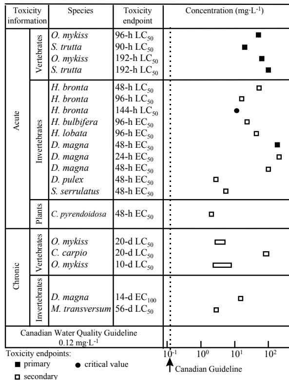
Figure 1. Select freshwater toxicity data for inorganic fluorides.
